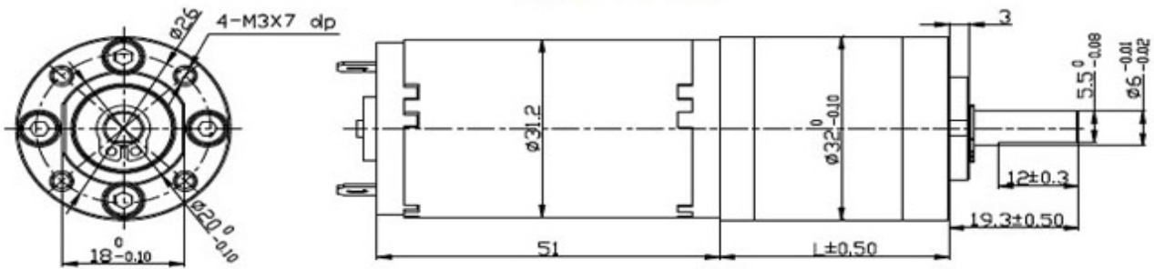
Outside Dimension
