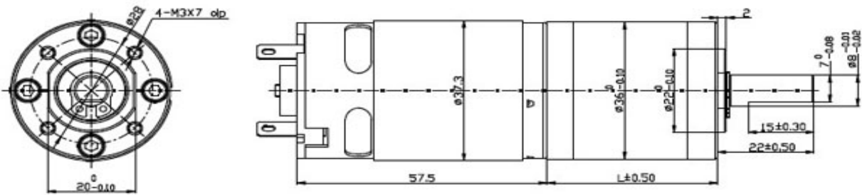
Outside Dimension
